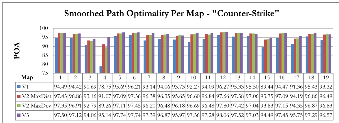
Figure 8.18: Per-map SGA* path optimality measurements for the "Counter-Strike" test set
