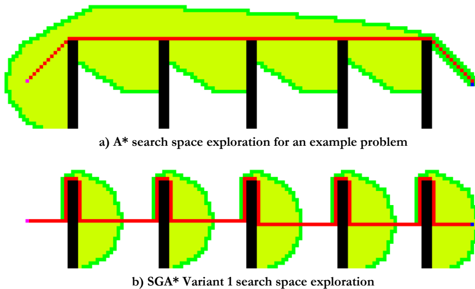
Figure 8.9: Unnecessary SGA* variant 1 search space exploration due to naïve sub-goal selection
