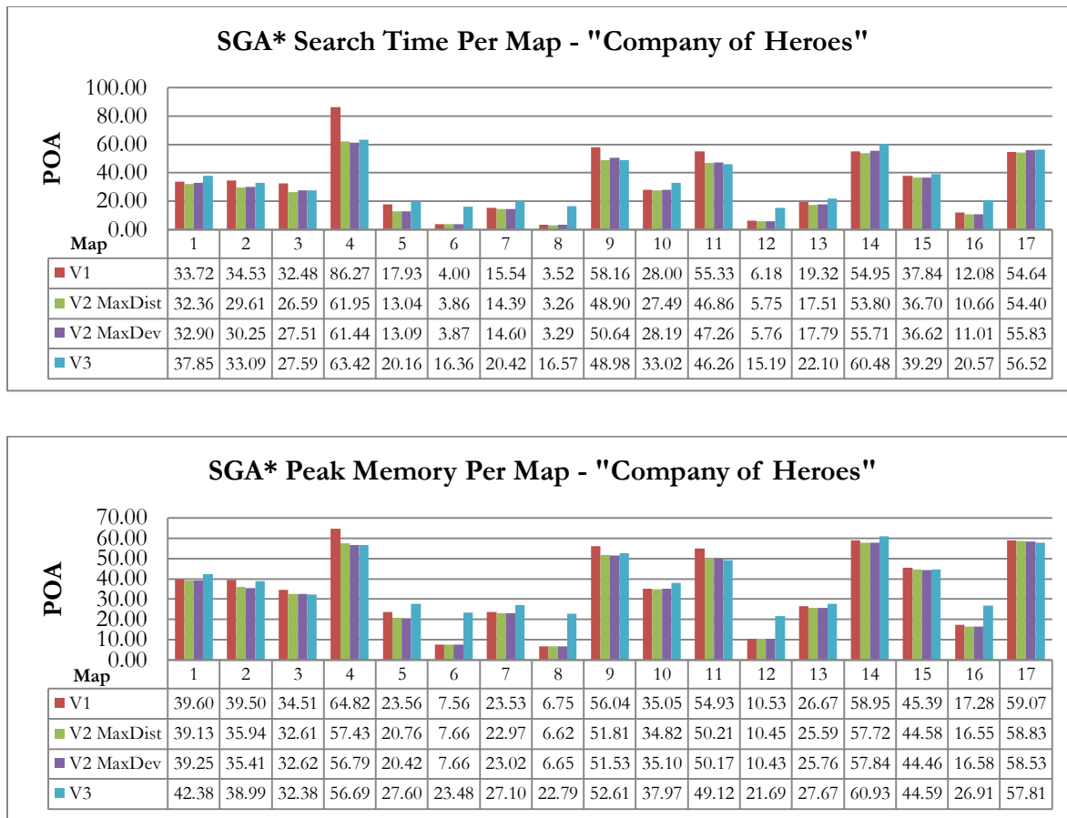
Figure 8.21: Per-map SGA* performance results for the "Company of Heroes" test set
