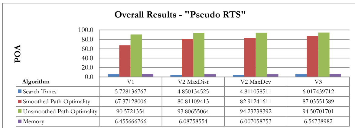
Figure 8.38: Overall SGA* results for the "Pseudo RTS" test set
