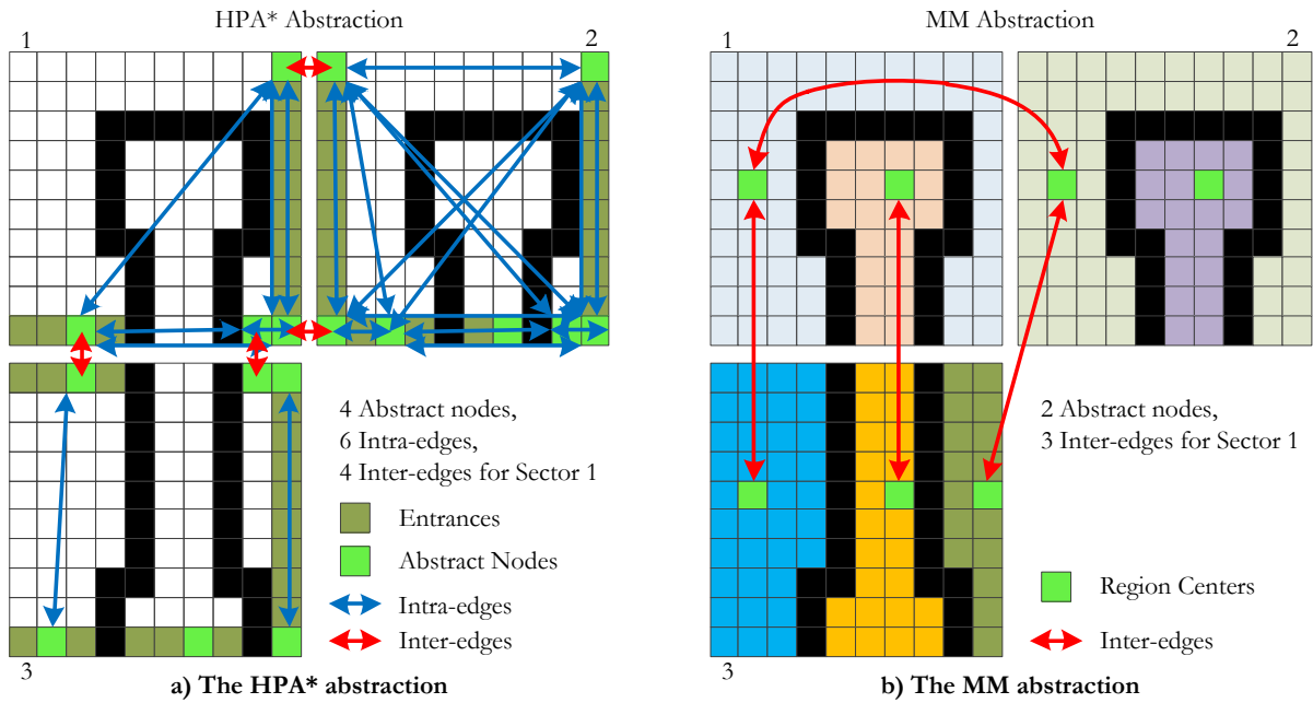
Figure 7.8: A comparison between the HPA* and MM* abstractions. (a). (b).
