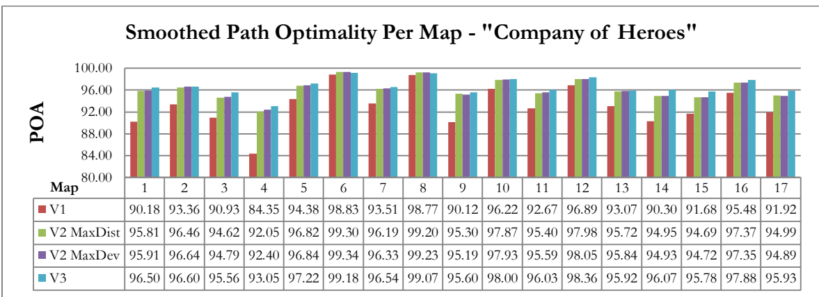
Figure 8.22: Per-map SGA* path optimality measurements for the "Company of Heroes" test set
