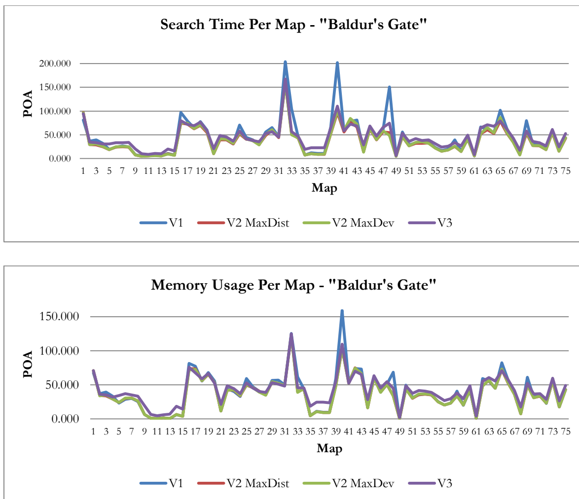
Figure 8.25: Per-map SGA* performance results for the "Baldur’s Gate" test set
