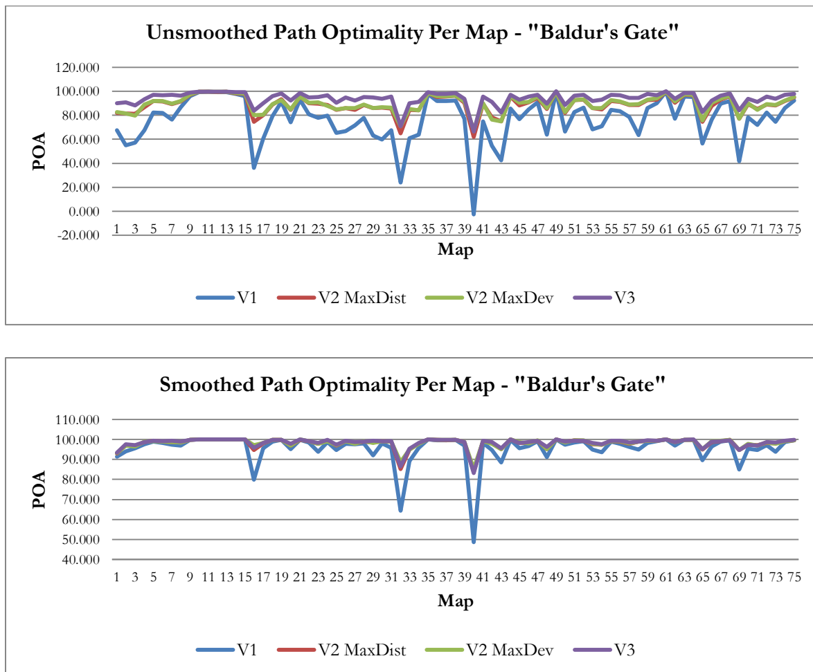
Figure 8.27: Per-map SGA* path optimality measurements for the "Baldur's Gate" test set
