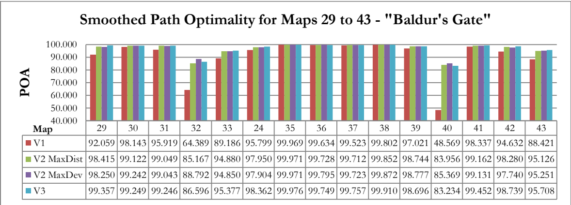
Figure 8.28: Per-map SGA* path optimality measurements for maps 29 to 43 of the "Baldur's Gate" test set
