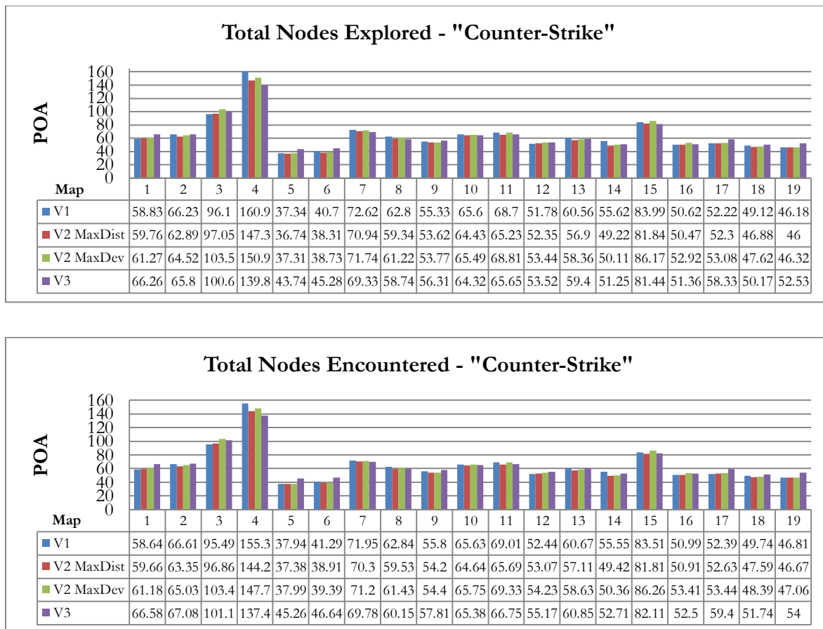
Figure 8.17: Search space exploration statistics for SGA* over A*
