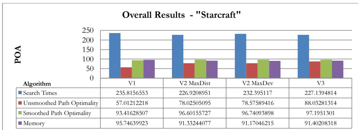
Figure 8.34: Overall SGA* results for the "Starcraft" test set
