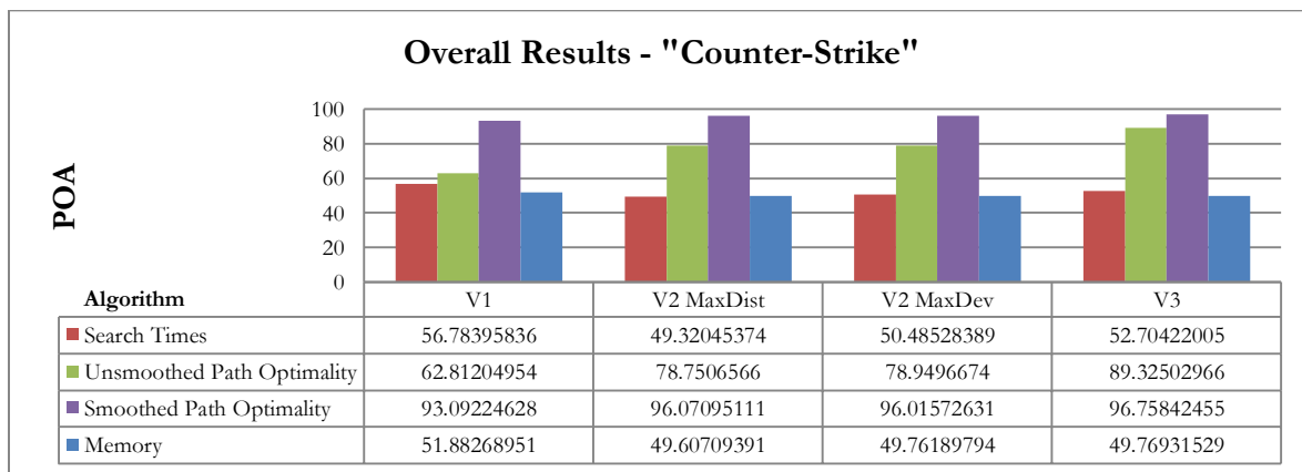
Figure 8.19: Overall SGA* results for the "Counter-Strike" test set
