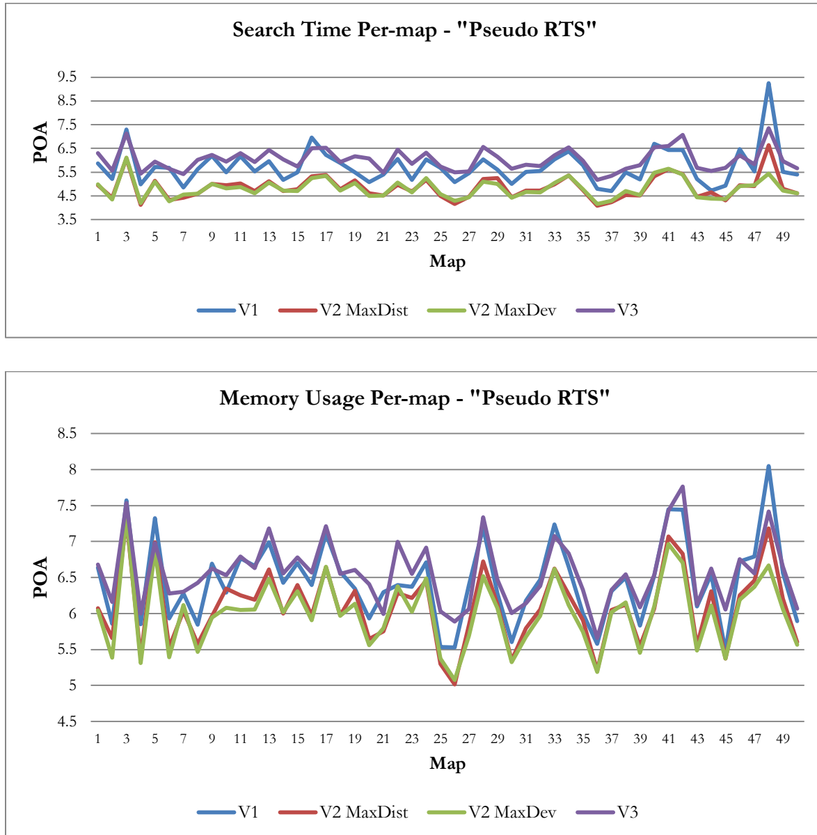
Figure 8.36: Per-map SGA* performance measurements for the "Pseudo RTS " test set
