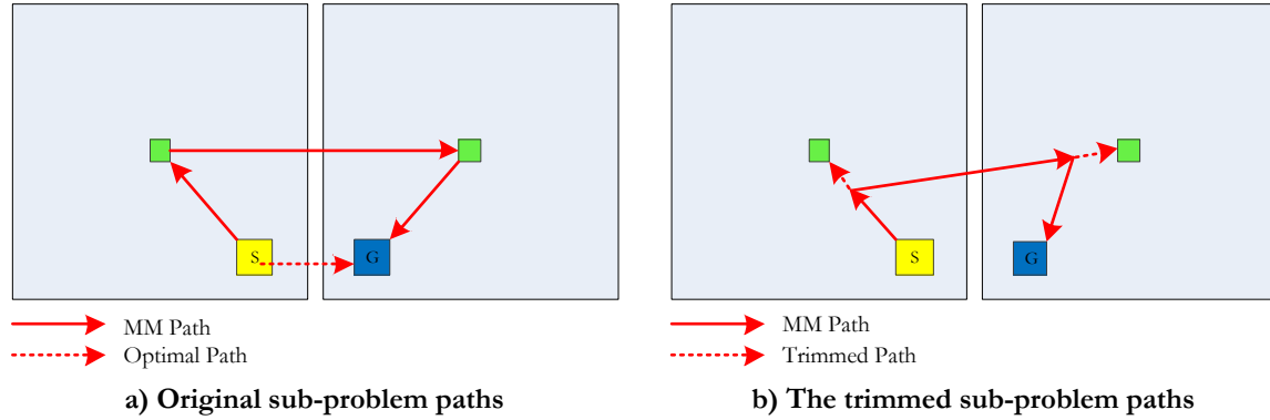
Figure 7.9: Improving path sub-optimality through the trimming of sub-problem solutions
