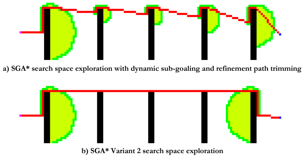
Figure 8.10: SGA* Variant 2 Search Space Exploration
