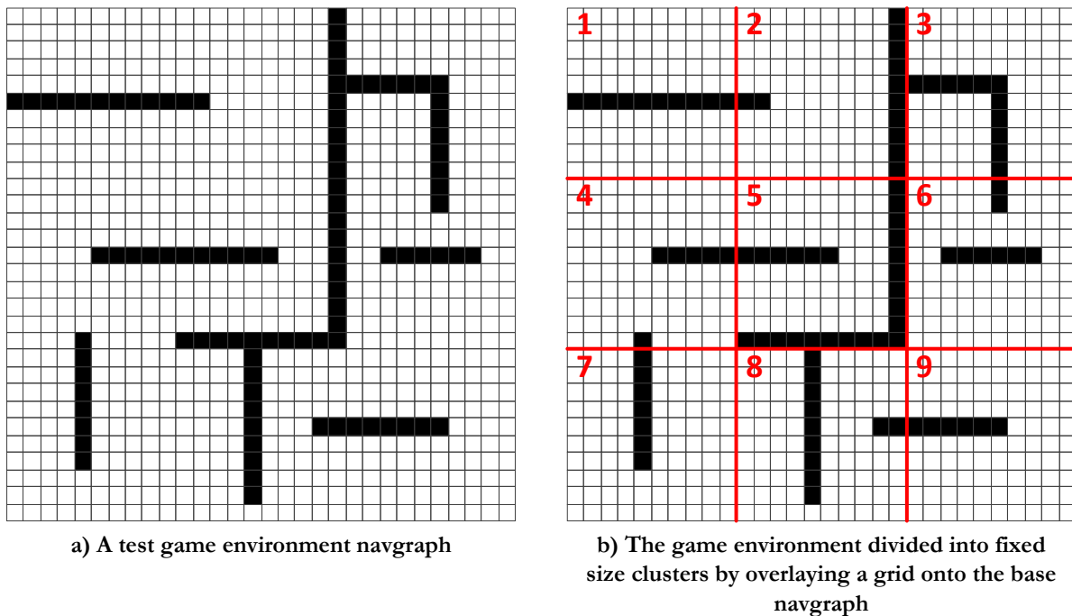
Figure 7.3: The HPA* graph abstraction cluster creation
