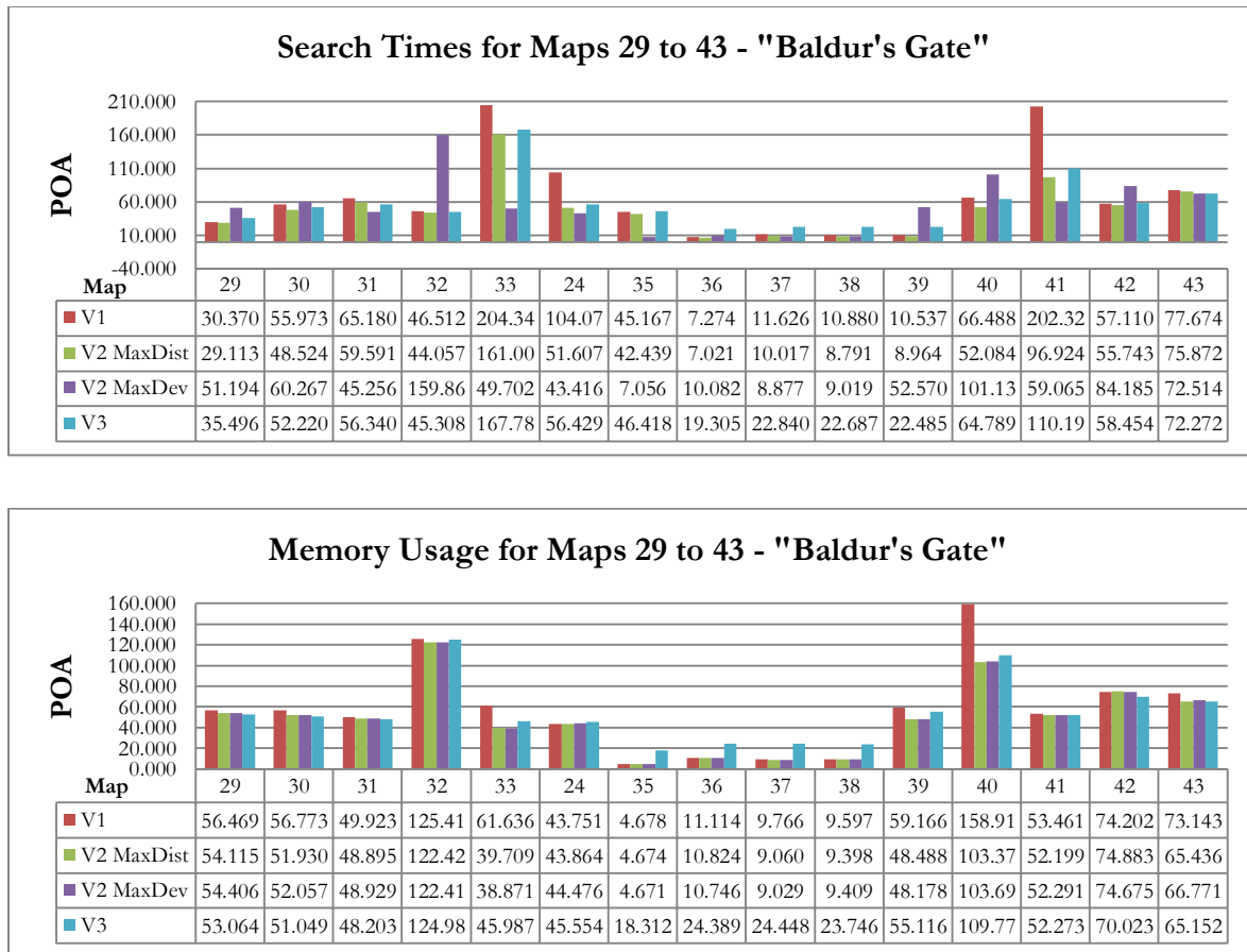
Figure 8.26: Per-map SGA* performance results for maps 29-43 of the "Baldur's Gate" test set
