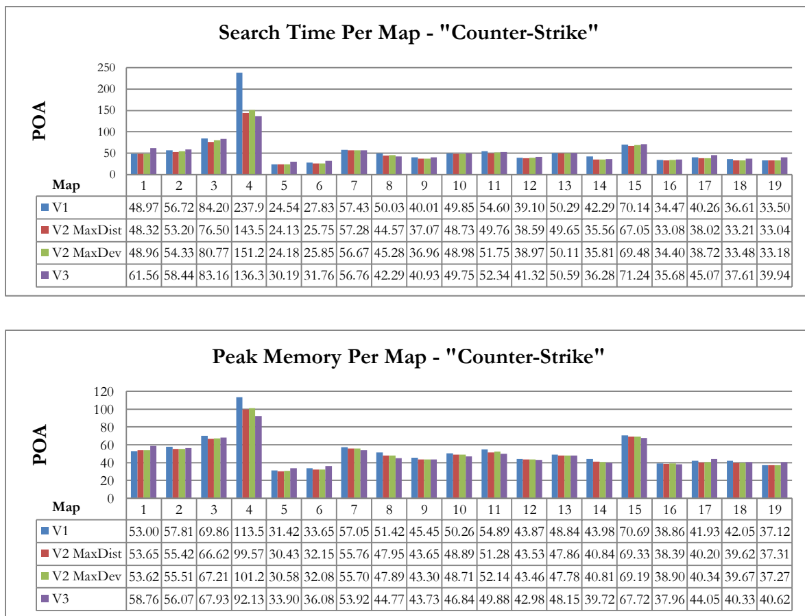
Figure 8.16: Per-map SGA* performance results for the "Counter-Strike" test set
