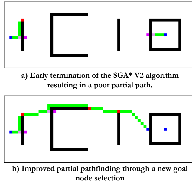
Figure 8.13: SGA* V2 Partial Pathfinding
