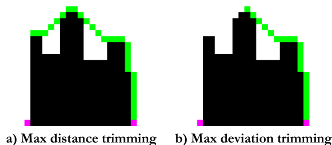
Figure 8.11: The difference between the two refinement path trimming techniques
