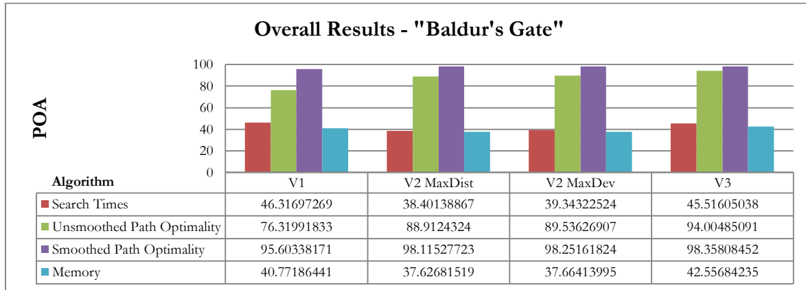
Figure 8.30: Overall SGA* results for the "Baldur's Gate" test set
