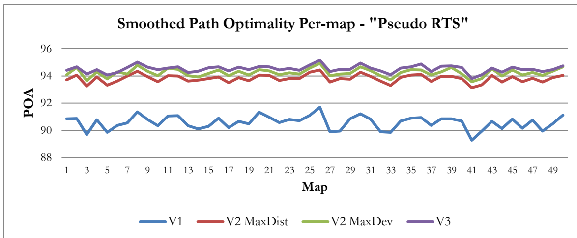
Figure 8.37: Per-map SGA* path optimality measurements for the "Pseudo RTS" test set
