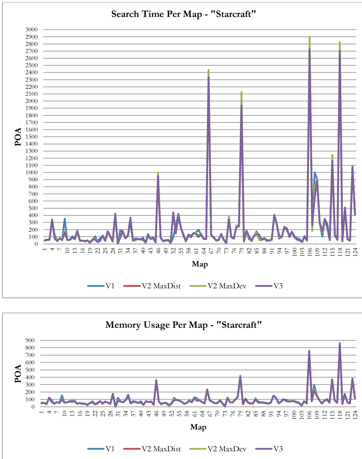
Figure 8.32: Per-map SGA* performance measurements for the "Starcraft" test set
