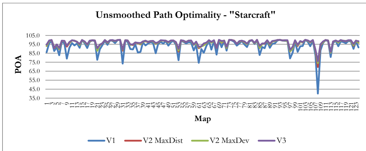
Figure 8.33: Per-map SGA* path optimality measurements for the "Starcraft" test set
