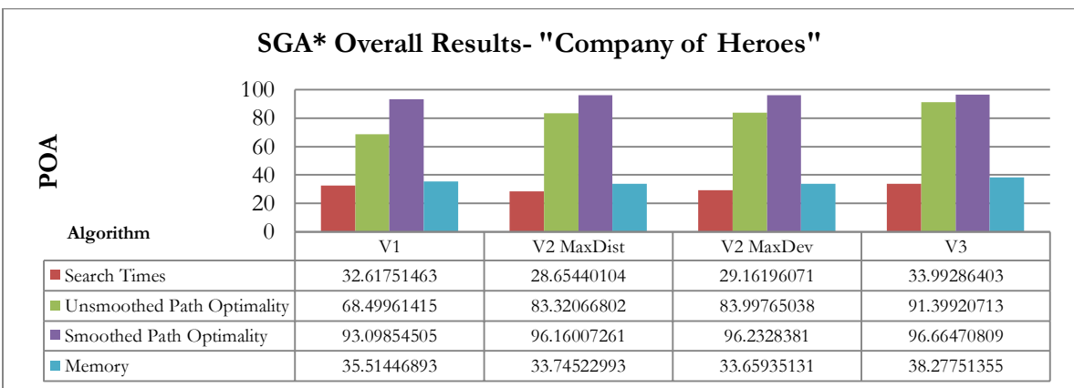
Figure 8.23: Overall SGA* results for the "Company of Heroes" test set
